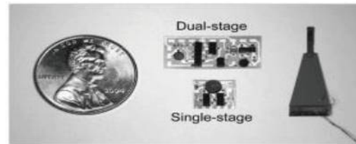
Fig.10. Implementations of piezoelectric drive circuits next to piezoelectric bimorph actuator [5]
