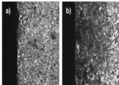
Fig. 14. Top view of ferrite edge manufactured using traditional sintering processes (a) and laser micromachining (b) under identical lighting conditions at 50X magnification (scale bars 40µm)
