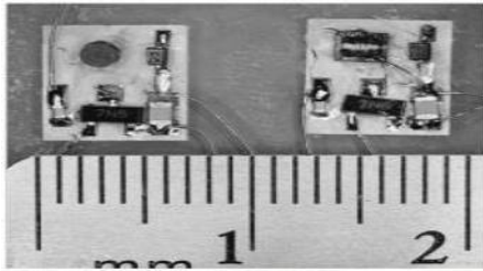
Fig.11. Implementations of the tapped inductor boost converter using bobbin core (left) and laser micromachined core (right). All other circuit components are kept the same
