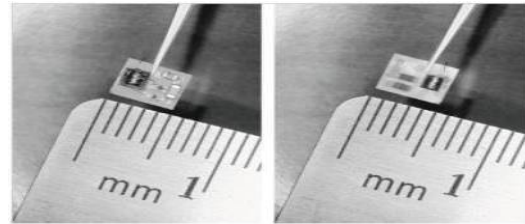
Fig. 15. Front and back view of 20mg tapped inductor boost converter
