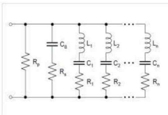
Fig.3. Piezoelectric element equivalent circuit
