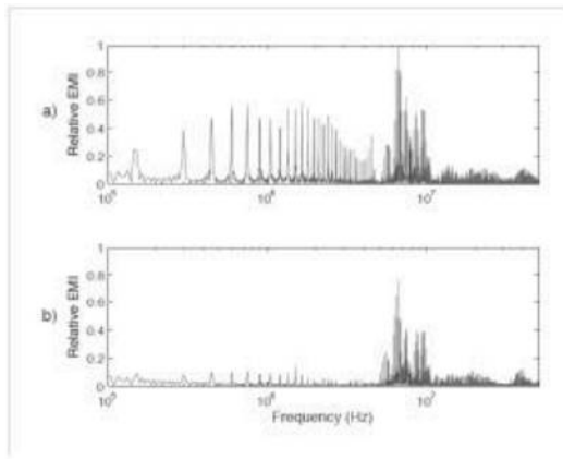
Fig. 13. Relative EMI spectra measured 1cm from bobbin core (a) and E-core (b)
