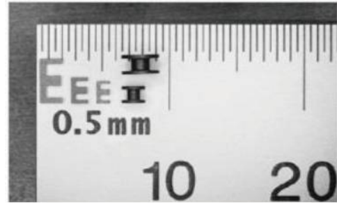
Fig.6. E-cores fabricated by laser micromachining and bobbin cores salvaged from commercial inductors
