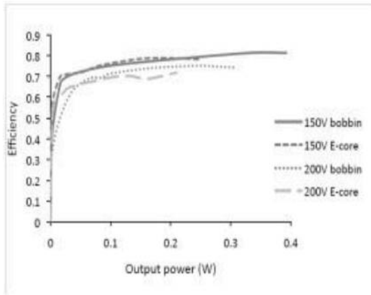
Fig. 12. Efficiency vs. output power of tapped inductor boost converters using bobbin core and laser micromachined E-core
