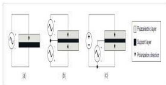
Fig.4. Unipolar drive methods for piezoelectric actuators: unimorph (a), bimorph with alternating drive (b), and bimorph with simultaneous drive (c)
