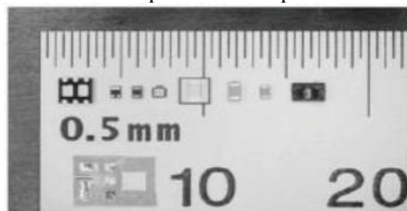
Fig.8. Chip-scale, bare-die, and passive components used in ultralight high-voltage power circuits. Left to right: Dual 190V nFETs, 30V nFET, 325V diode, bare-die 240V nFET (decapsulated with sulfuric acid), bare-die 60V nFET (commercially available), 0.1µF 200V capacitor, 4.2µF 6.3V capacitor, 5mg laser micromachined inductor. Bottom: Flex circuit substrate manufactured from DuPont Pyralux laminate
