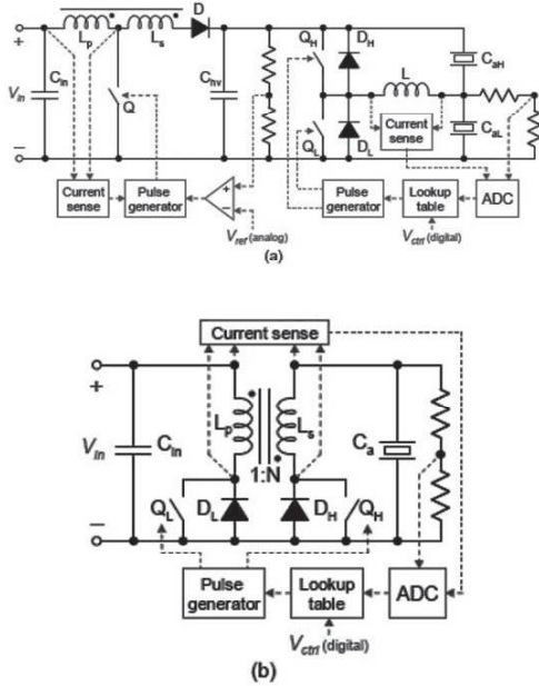
Fig.5. Lightweight circuit topologies suitable for driving piezoelectric actuators
