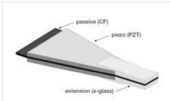
Fig. 2. Piezoelectric bimorph structure.
