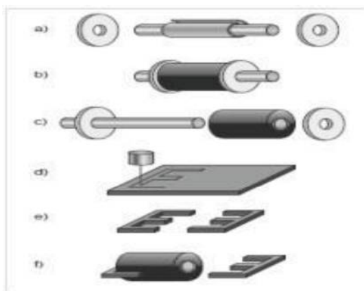
Fig.7. Fabrication of custom magnetic components: a) temporary bobbin formation using Kapton liner and laser-cut plastic discs, b) coil winding, c) temporary bobbin removal, d) laser micromachining of ferrite core, e) core release, f) component assembly
