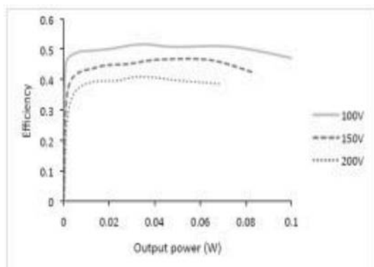
Fig. 16. Efficiency vs. output power of 20mg tapped inductor boost converter at three output voltage levels
