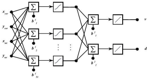
Fig.2. Schematic representation of the proposed model of the ANN
