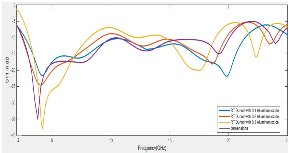
Fig.3. S11 plot of conventional antenna and antenna with substrates of RT Duriod 5880 with 0.1 Aluminum Oxide, 0.2 Aluminum Oxide and 0.3 Aluminum Oxide
