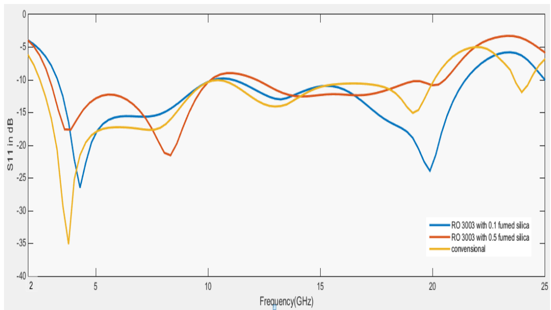
Fig.4. S11 plot of conventional antenna and antenna with substrate of RO3003 with 0.1 and 0.5 fumed silica
