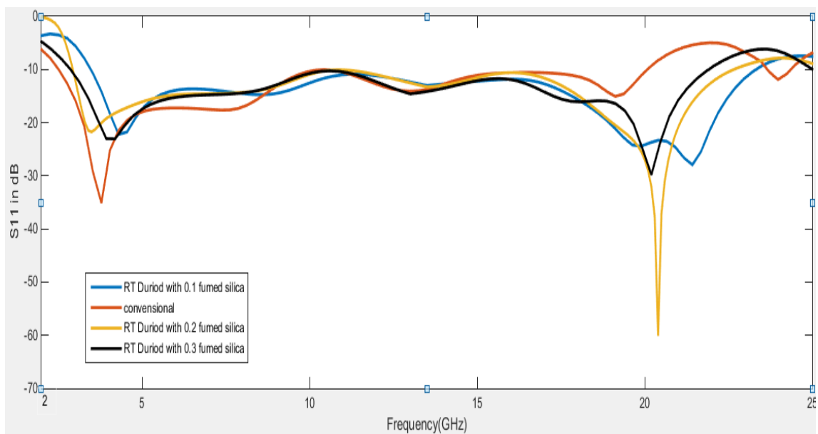
Fig.2. S 11 plot of conventional antenna and antenna with substrates of RT Duriod 5880 with 0.1 Fumed Silica, 0.2 Fumed Silica and 0.3 Fumed Silica
