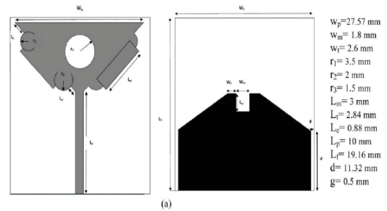
Fig.1. Configuration and parameters of proposed antenna
