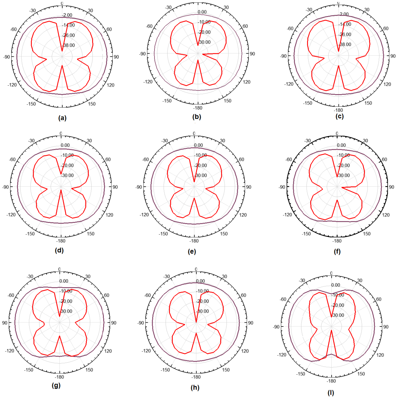
Fig.5. Radiation pattern of the antenna in E- plane a) conventional antenna (b) antenna with substrate of RT Duriod 5880 with 0.1 fumed silica (c) RT Duriod 5880 with 0.2 fumed silica (d) RT Duriod 5880 with 0.3 fumed silica (e) RT Duriod 5880 with 0.1 Aluminum oxide (f) RT Duriod 5880 with 0.2 Aluminum oxide (g) RT Duriod 5880 with 0.3 aluminum oxide (h) RO3003 with 0.1 fumed silica (I) RO3003 with 0.5 fumed silica at 12 GHz.
